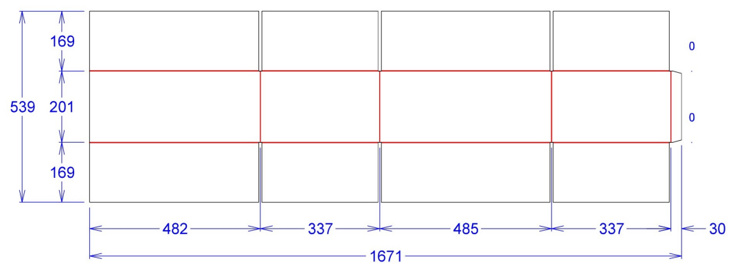
Outer Case Line Drawing:
